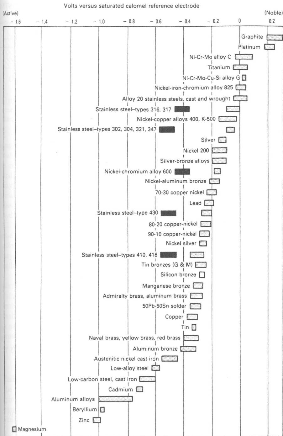
Figure 13 The galvanic series for metals immersed in flowing seawater. (From Ref. 8, with permission from ASM International.)
